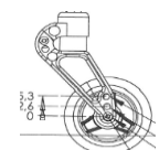
Frog leg design 149 mm x 41 mm
